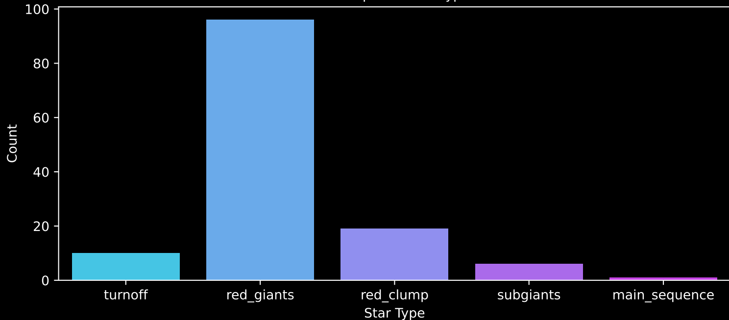
APOGEE DR17 Field: [SGRCMA-04] Count plot of Star Type
