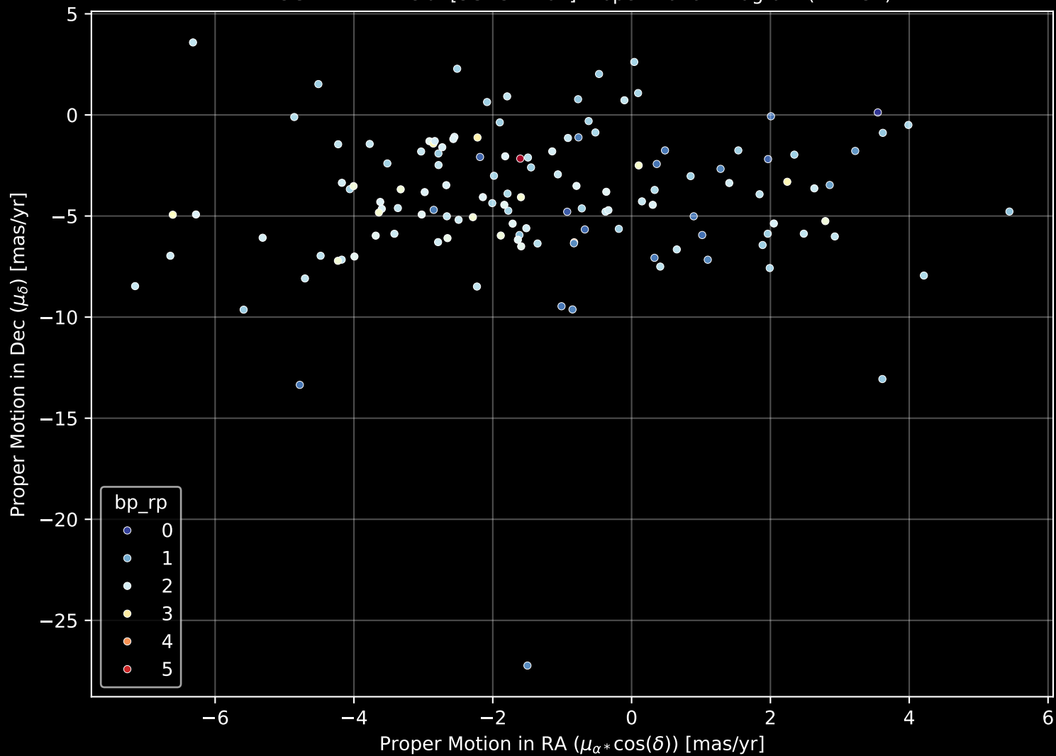
APOGEE DR17 Field: [SGRCMA-04] Proper Motion Diagram (n= 132)
