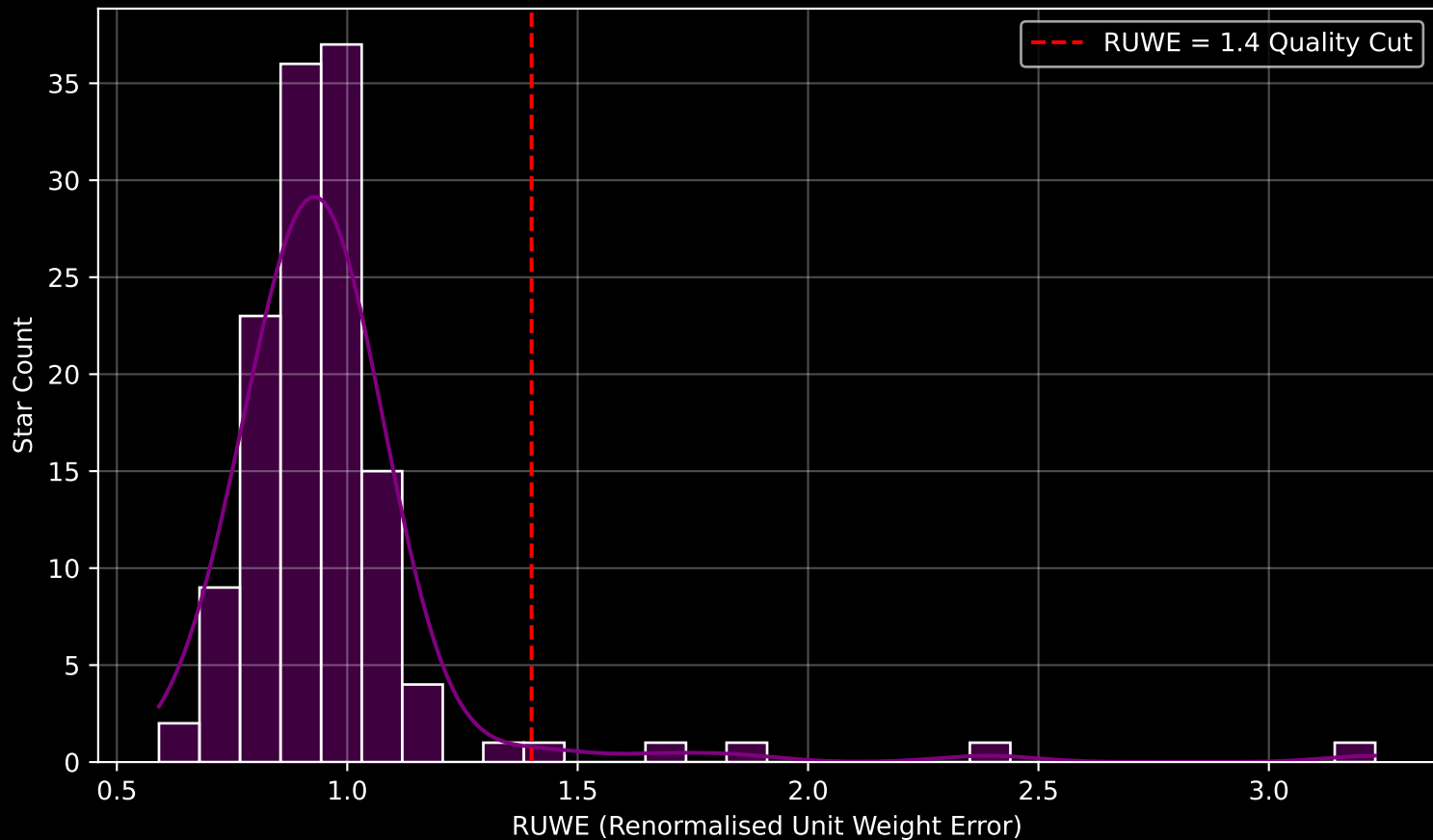
GAPOGEE DR17 Field [SGRCMA-04] RUWE Distribution (n= 132)
