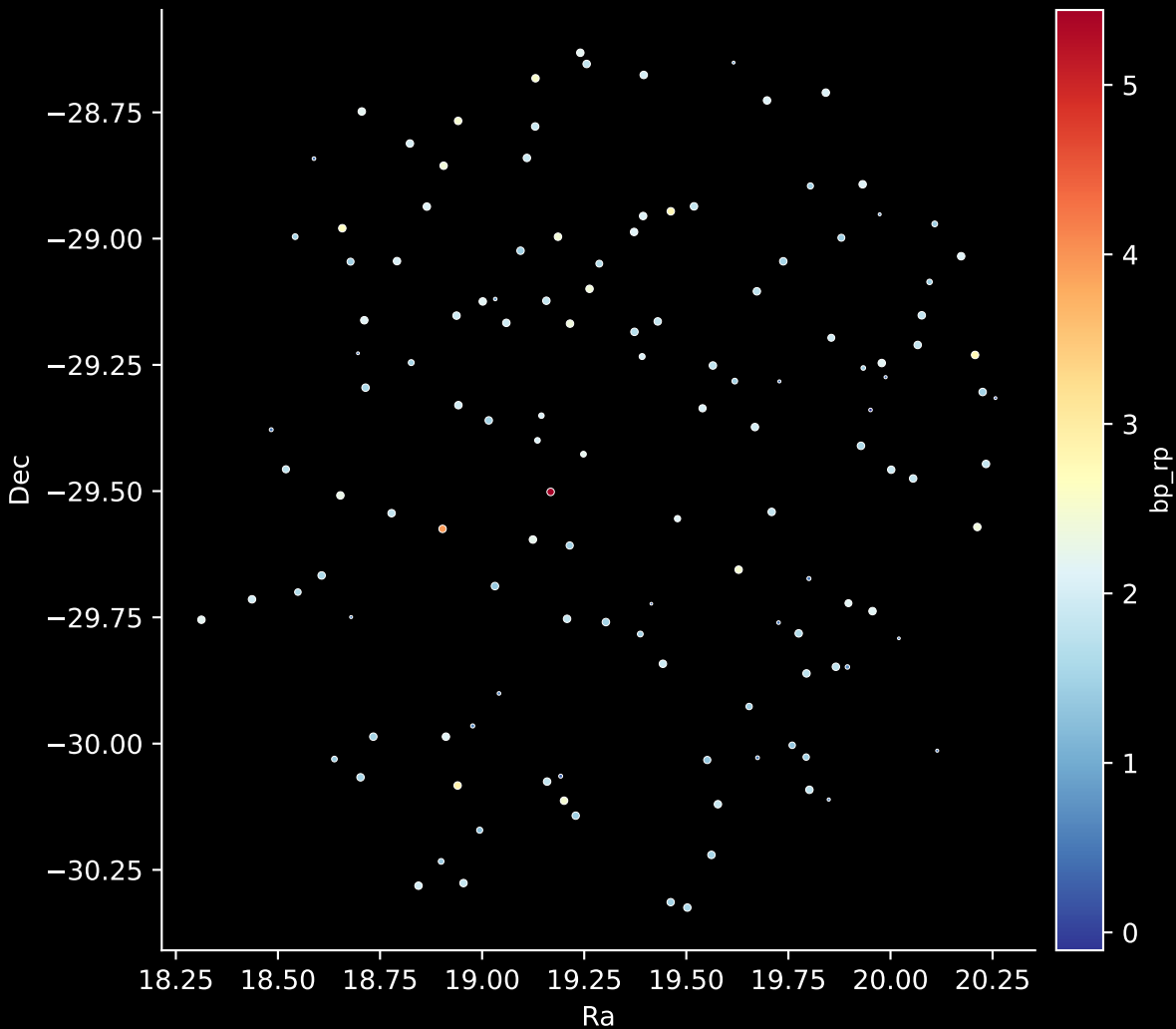
APOGEE DR17 Field: [SGRCMA-04] Stars: 132
