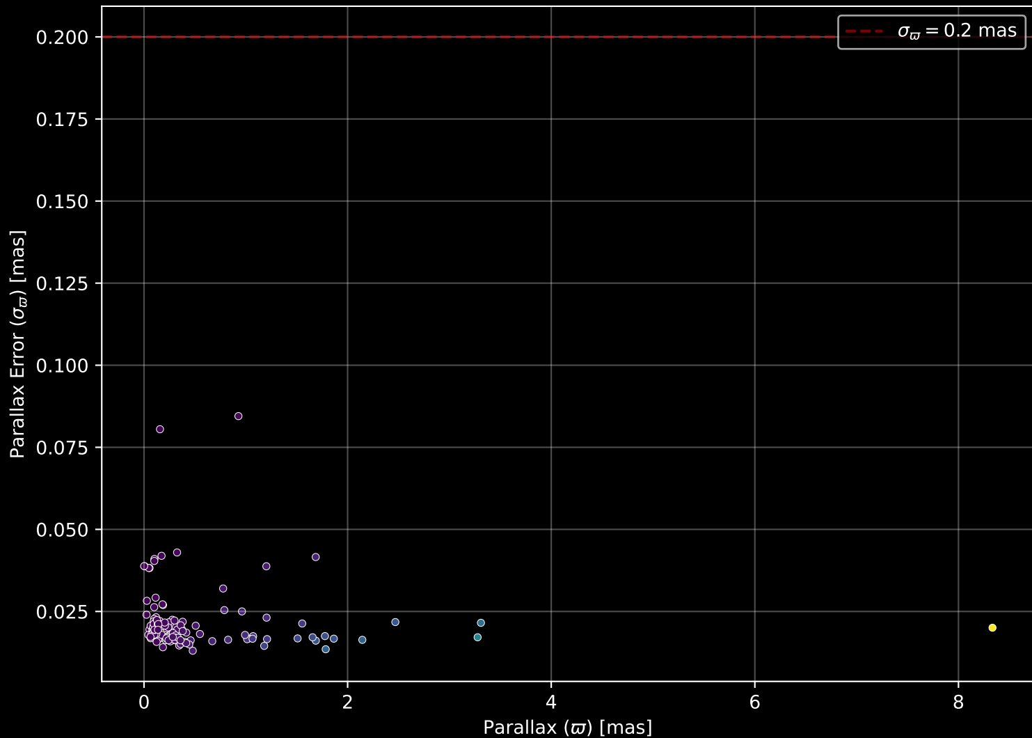
APOGEE DR17 Field: [SGRCMA-04] Parallax Quality (n= 132)
