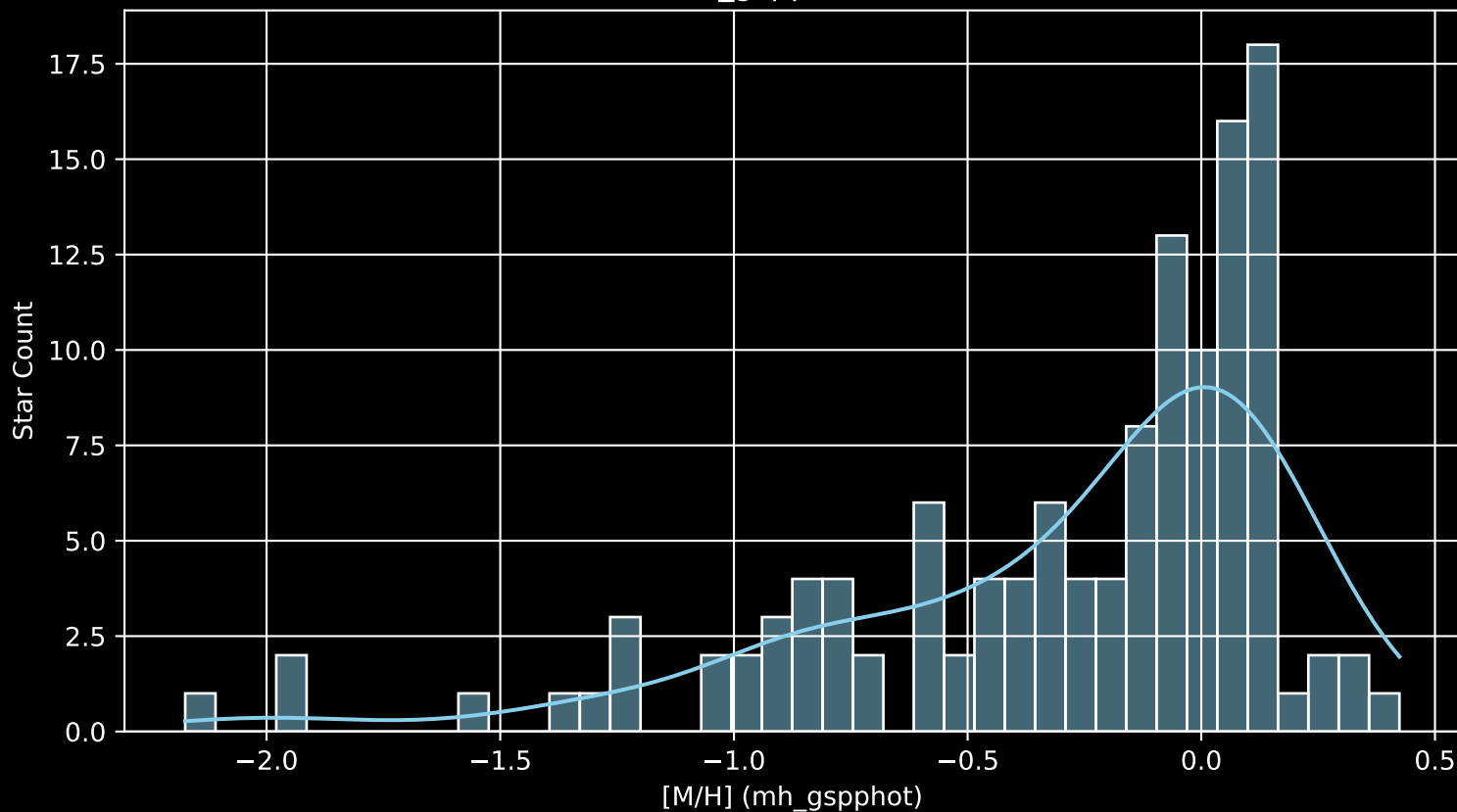
APOGEE DR17 Field: [SGRCMA-04 [M/H] (mh_gspphot) (n= 127)
