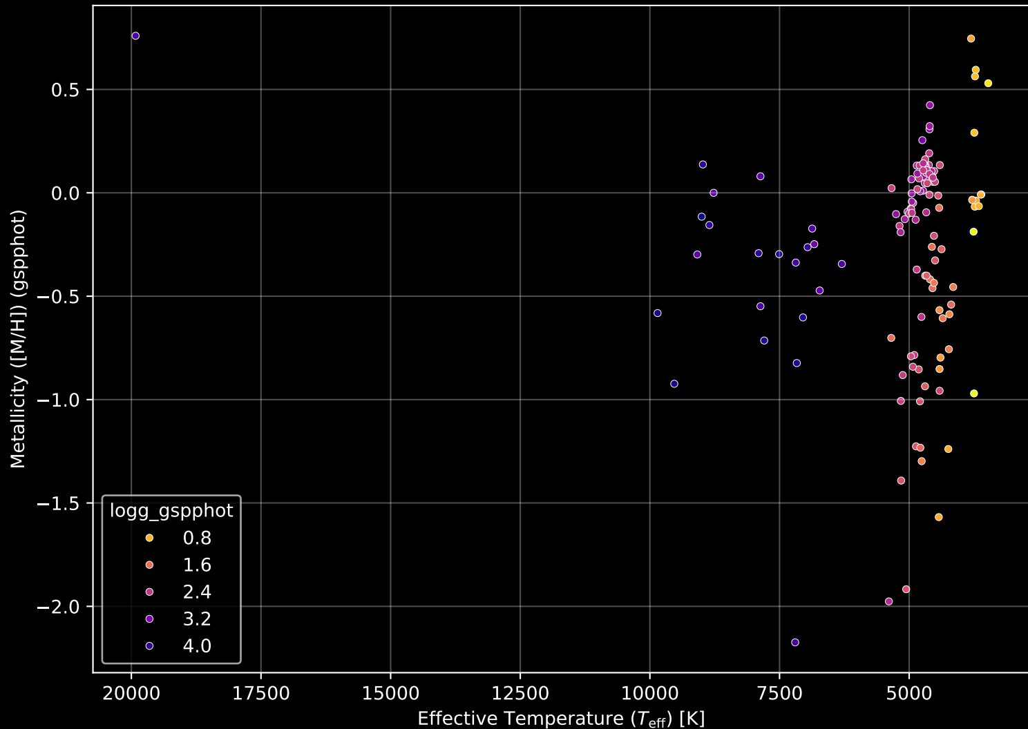
APOGEE DR17 Field: [SGRCMA-04] Stellar Population Parameters (n= 132)
